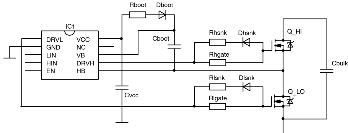
Figure 48. Recommended Schematic
