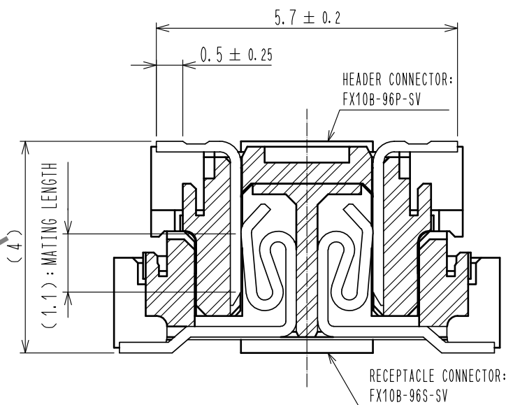
CROSS CUT SECTION (10:1)
