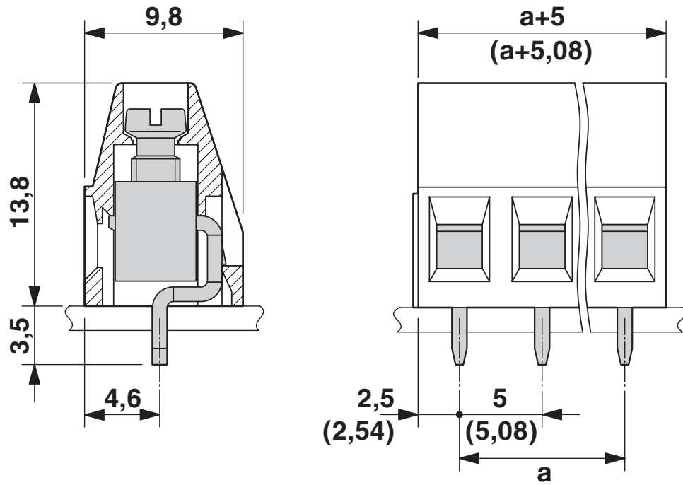
Dimensional drawing
