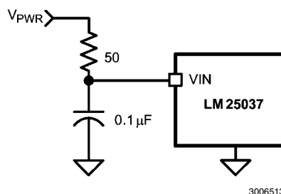
FIGURE 10. Input Transient Protection
