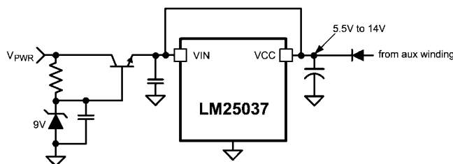
FIGURE 11. Start-up Regulator for V_{PWR} > 75V
