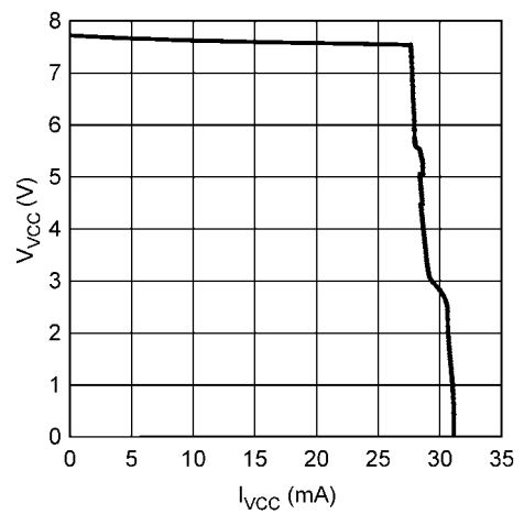
V_{VCC} vs I_{VCC}
