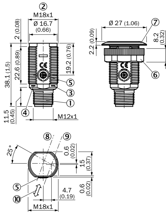
GRTB18S, plastic, connector, straight, adjustable
