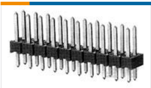
TE Part #1-826632-6 16P AMPMODU II STIFT LEI
