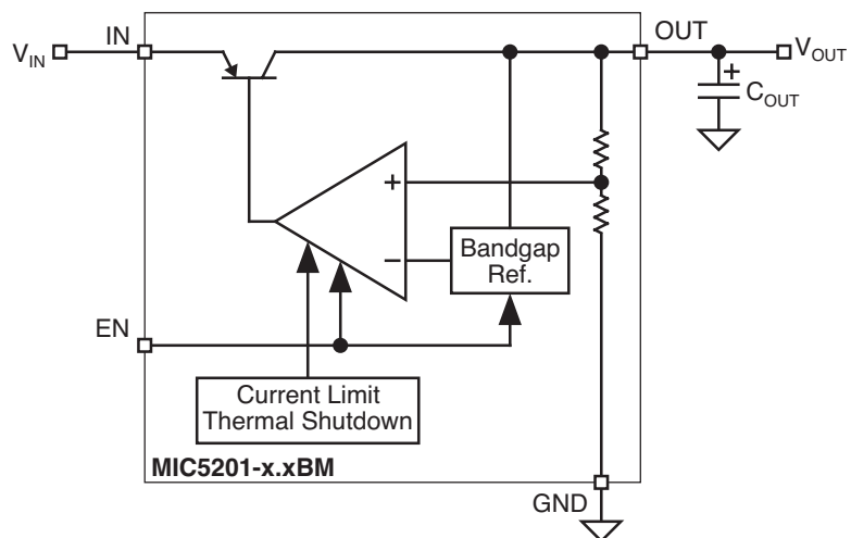
Fixed Regulator
