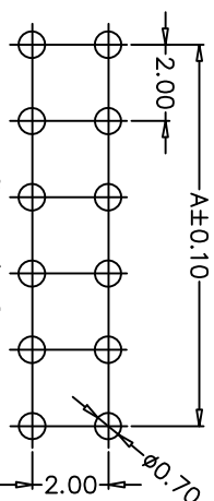
PCB LAYOUT
