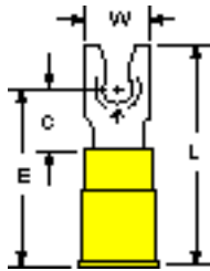
MNG10-6FL 6 12-10
