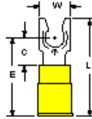
MNG10-10FL 10 12-10
