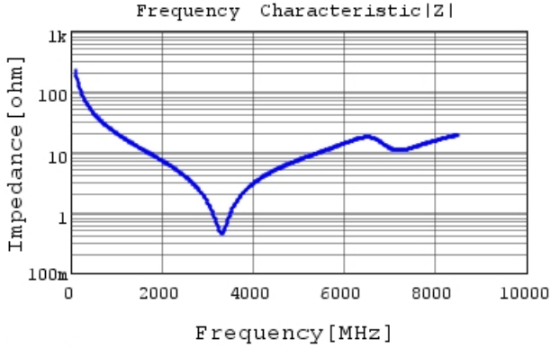
GRM1555C2A7R2WA01 |Z| DCOV, 25degC
