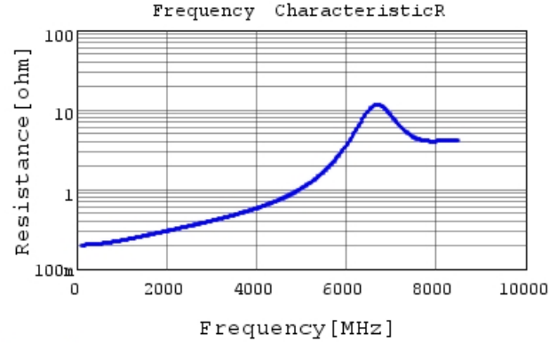
GRM1555C2A7R2WA01 R DCOV, 25degC
