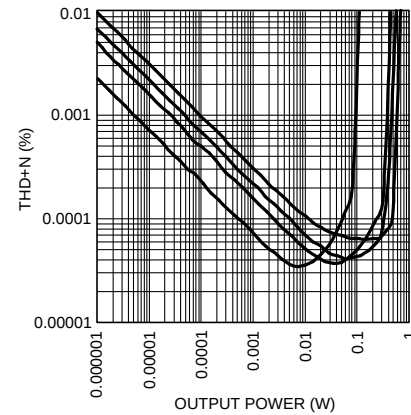
Figure 8. THD+N vs Output Power LME49720/LME49600 headphone amplifier into (from top to bottom at 10mW): 16Ω, 32Ω, 64Ω, 300Ω ( V_s = \pm 9V , f = 100\text{Hz} , 22\text{Hz} \leq \text{BW} \leq 22\text{kHz} )
