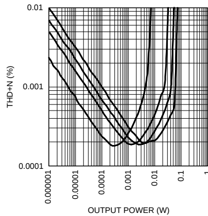
Figure 7. THD+N vs Output Power LME49720/LME49600 headphone amplifier into (from top to bottom at 0.1mW): 16Ω, 32Ω, 64Ω, 300Ω ( V_s = \pm 3V , f = 100\text{Hz} , 22\text{Hz} \leq \text{BW} \leq 22\text{kHz} )
