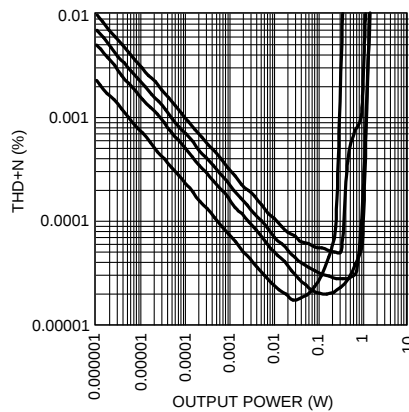
Figure 9. THD+N vs Output Power LME49720/LME49600 headphone amplifier into (from top to bottom at 10mW): 16Ω, 32Ω, 64Ω, 300Ω ( V_s = \pm 15V , f = 100\text{Hz} , 22\text{Hz} \leq \text{BW} \leq 22\text{kHz} )
