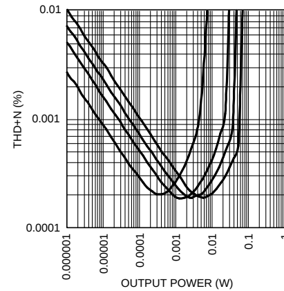
Figure 10. THD+N vs Output Power LME49720/LME49600 headphone amplifier into (from top to bottom at 0.1mW): 16Ω, 32Ω, 64Ω, 300Ω ( V_s = \pm 3V , f = 1\text{kHz} , 400\text{Hz} \leq \text{BW} \leq 22\text{kHz} )
