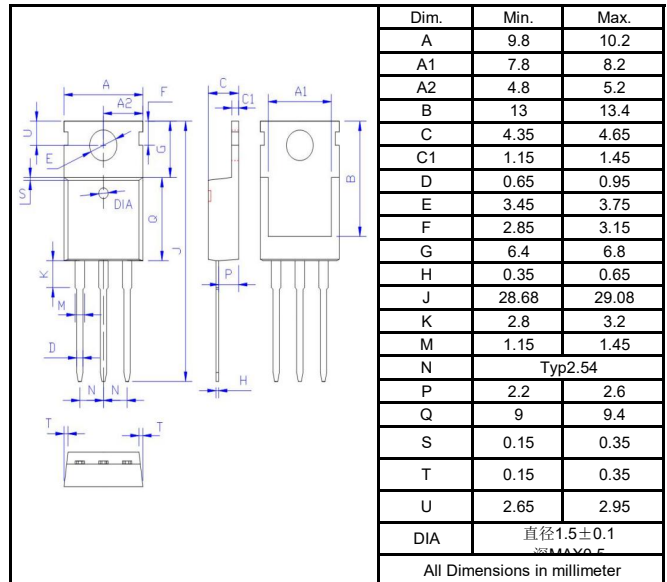
T0-220C
