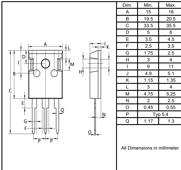
T0-247S
