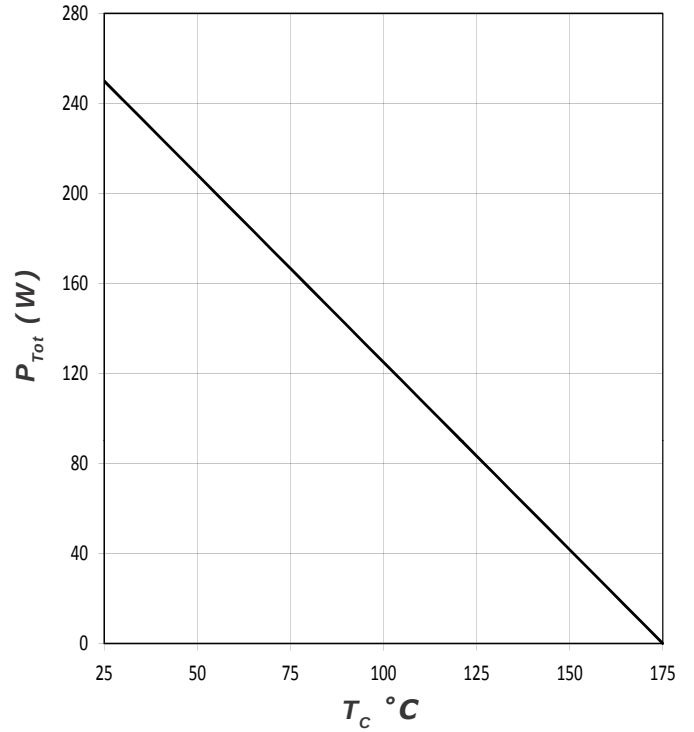
Figure 4. Power Derating
