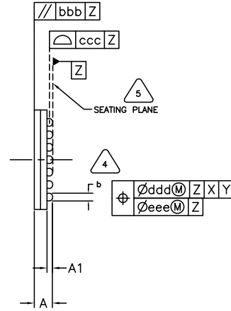
Figure 18. 50-Ball WFBGA Mechanical Drawing
