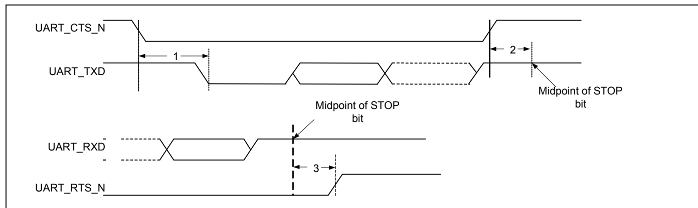
Figure 12. UART Timing
