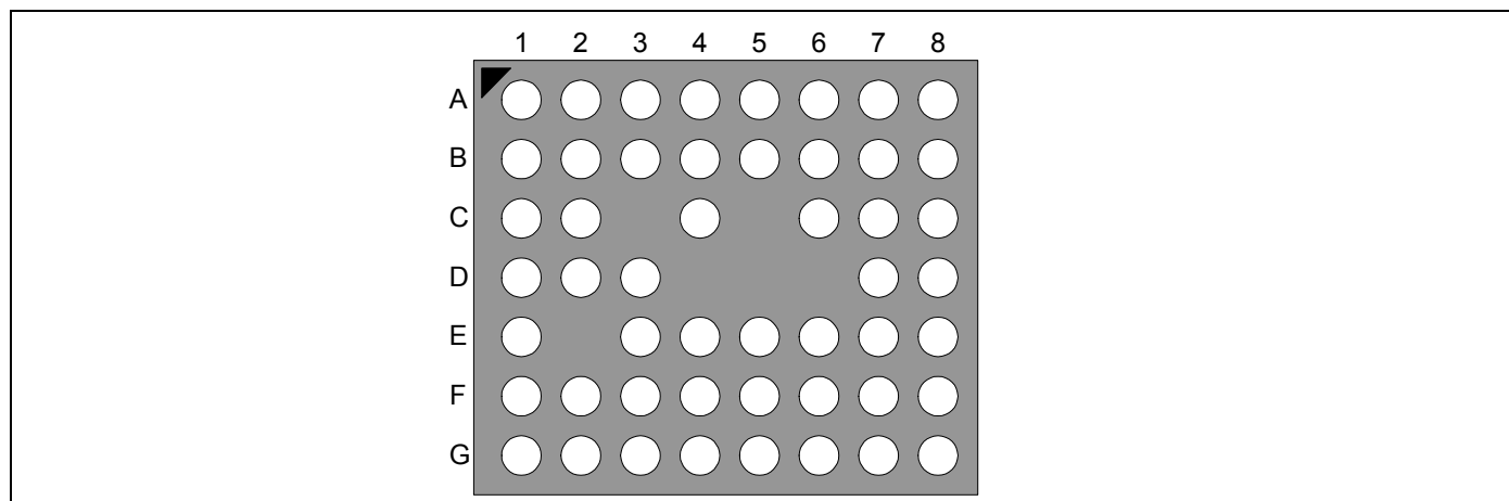
Figure 9. 4.5 x 4 x 0.8 mm (WFBGA) Array
