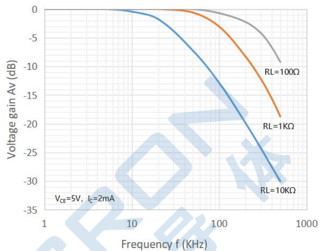
Fig.8 Frequency Response
