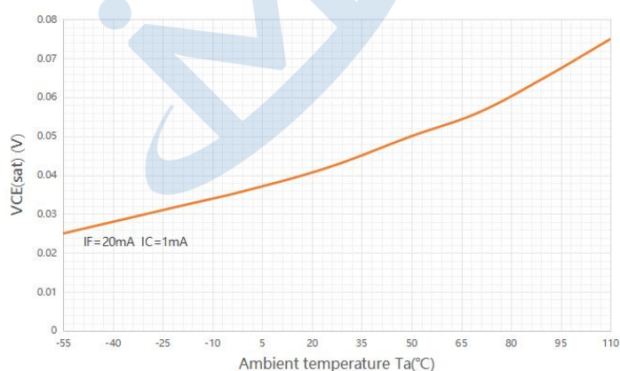
Fig.5 Collector-emitter Saturation Voltage vs. Ambient Temperature
