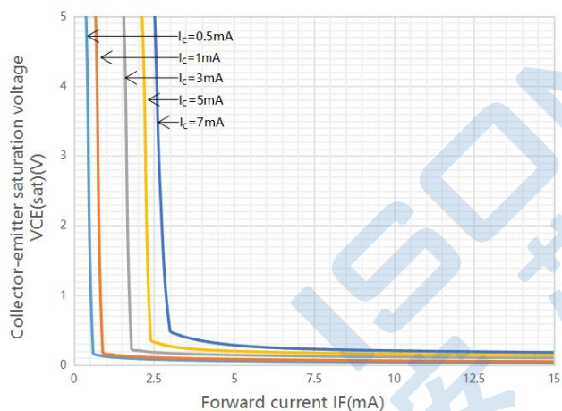
Fig.9 Collector-emitter Saturation Voltage vs Forward Current
