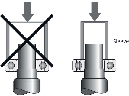
Fitting Bearing to Shaft
