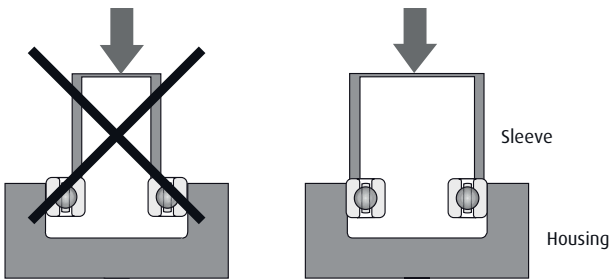
Fitting Bearing into Housing
