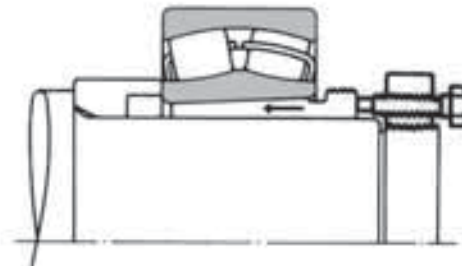
Mounting with Withdrawal Sleeve
