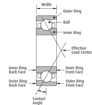
Single Row Angular Contact Ball Bearing
