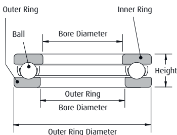
Single Direction Thrust Ball Bearing
