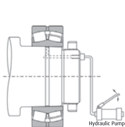
Removal Using Oil Injection
