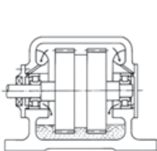
Splash Lubrication: gearboxes
