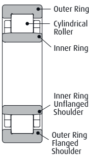
Cylindrical Roller Bearing (NU Style)
