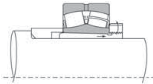
Mounting w/Adapter
