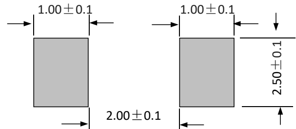
Recommended Pad Layout (mm)
