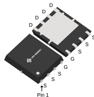
DFN5X6-8L (TDSON-8-EP(5x6))
