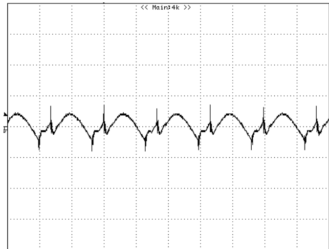
Figure 14: Output voltage ripple at nominal input voltage and rated load current ( I_o=4\text{A} ) ( 20\text{ mV/div} , 2\mu\text{s/div} ) Load capacitance: 1\mu\text{F} ceramic capacitor and 10\mu\text{F} tantalum capacitor. Bandwidth: 20\text{ MHz} . Scope measurements should be made using a BNC cable (length shorter than 20 inches). Position the load between 51 mm to 76 mm (2 inches to 3 inches) from the module.
