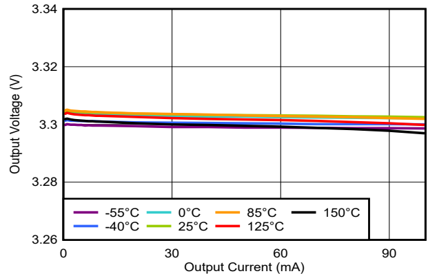
Figure 5-2. Load Regulation
