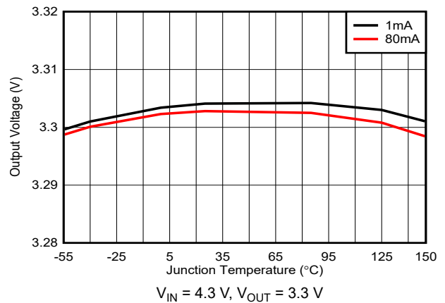
Figure 5-4. V_{OUT} vs Temperature and I_{OUT}
