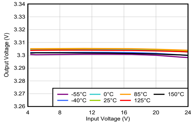
Figure 5-1. Line Regulation
