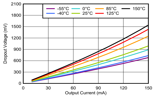
Figure 5-6. V_{DO} vs I_{OUT}
