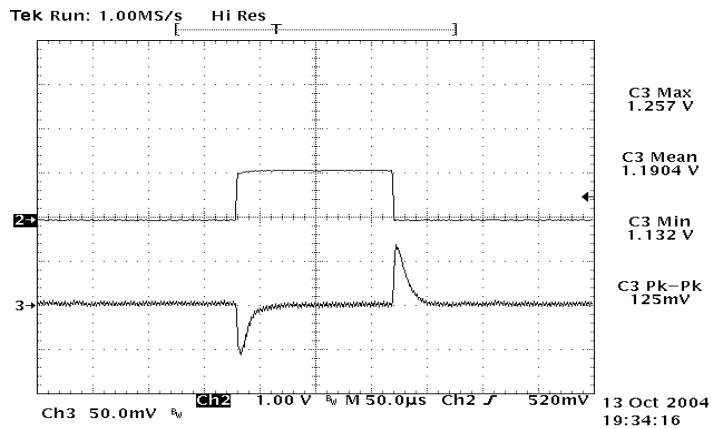
Figure 19: Typical transient response to step load change at 10A/\mu S from 75% to 50% of I_o , max at 12Vin, 1.2V out (Cout = 1μF ceramic, 10μF tantalum)
