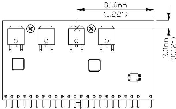
Figure 36: Temperature measurement location * The allowed maximum hot spot temperature is defined at 125 °C
