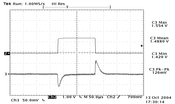
Figure 20: Typical transient response to step load change at 10A/\mu S from 75% to 50% of I_o , max at 12Vin, 1.5V out (Cout = 1μF ceramic, 10μF tantalum)
