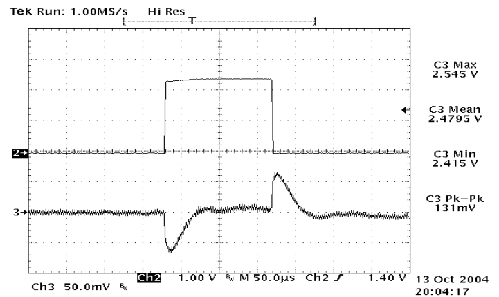
Figure 22: Typical transient response to step load change at 10A/\mu S from 75% to 50% of I_o , max at 12Vin, 2.5V out (Cout = 1μF ceramic, 10μF tantalum)
