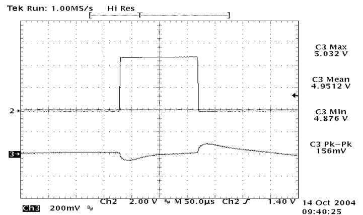
Figure 24: Typical transient response to step load change at 10A/\mu S from 75% to 50% of I_o , max at 12Vin, 5.0V out (Cout = 1μF ceramic, 10μF tantalum)
