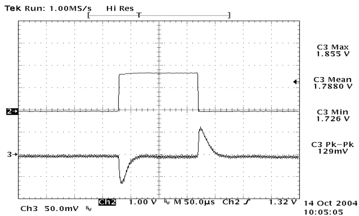
Figure 21: Typical transient response to step load change at 10A/\mu S from 75% to 50% of I_o , max at 12Vin, 1.8V out (Cout = 1μF ceramic, 10μF tantalum)
