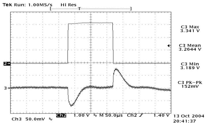
Figure 23: Typical transient response to step load change at 10A/\mu S from 75% to 50% of I_o , max at 12Vin, 3.3V out (Cout = 1μF ceramic, 10μF tantalum)
