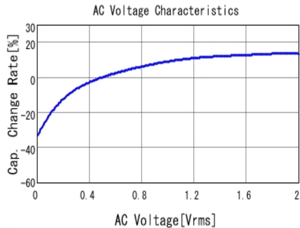
■ LLL153R60G224ME14 C-AC Voltage capchange, DC0V, 25.0d
