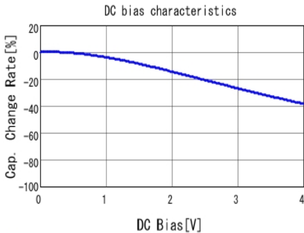
■ LLL153R60G224ME14 C-DC bias capchange, 25.0degC, AC0.
