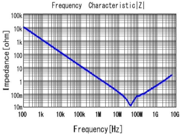
■ LLL153R60G224ME14 |Z| DC0V, 25degC
