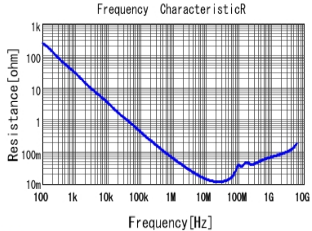
■ LLL153R60G224ME14 R DC0V, 25degC
