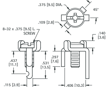
Mounting Detail
