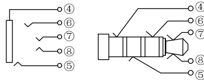
CIRCUIT DIAGRAM
