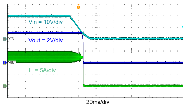
Figure 7-13. Shutdown Relative to VIN Falling, I_{OUT} = 5A
