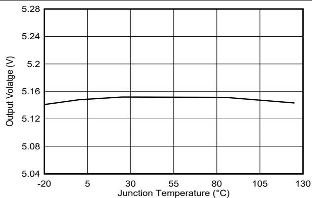
Figure 5-9. Output Voltage vs Junction Temperature
