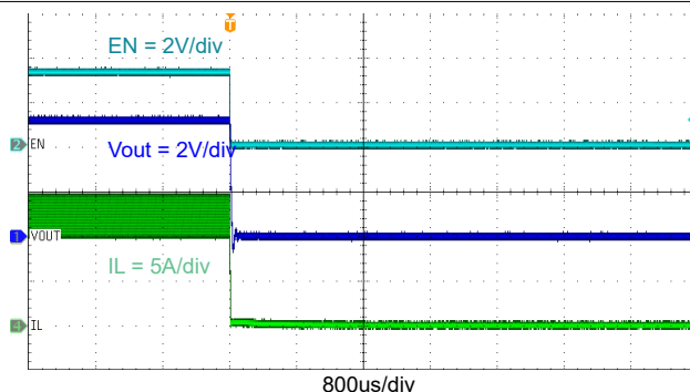
Figure 7-11. Shutdown Through EN, I_{OUT} = 12A
