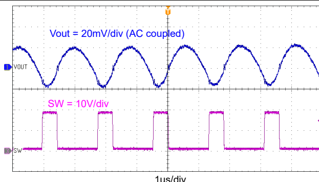
Figure 7-15. Output Voltage Ripple, I_{OUT} = 6A
