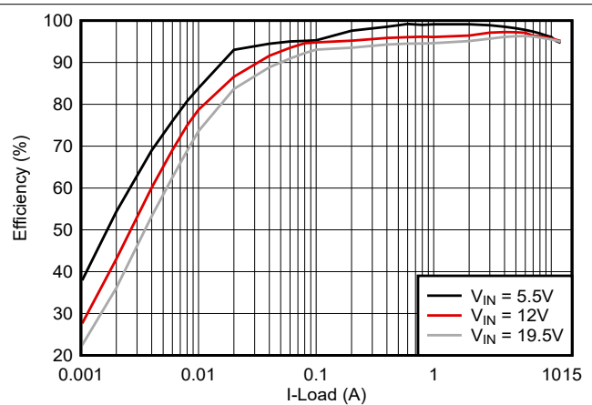
Figure 7-3. Efficiency Curve (OOA)
