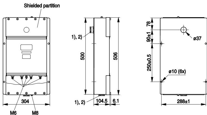
Drawing 8 - B84299D2060E003 (4x6A), B84299D2160E001 (4x16A)
