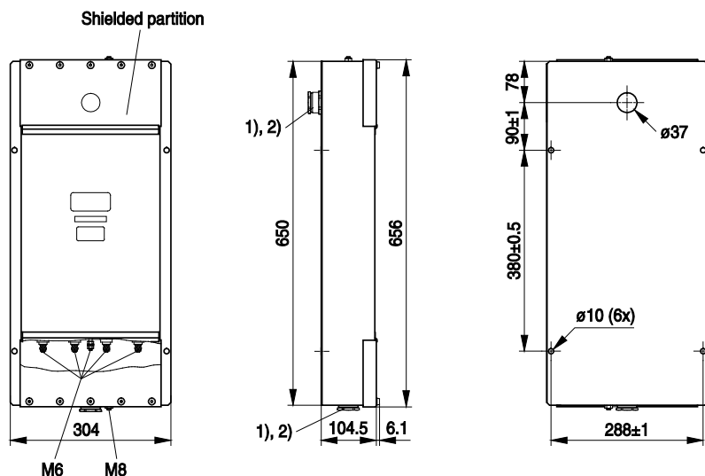
Drawing 12 - B84299D2320E001 (4x32A)
