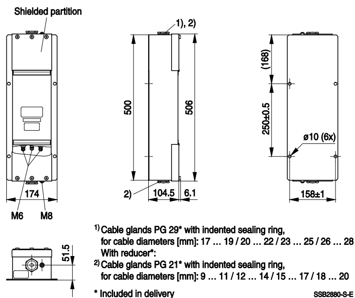
Drawing 1 - B84299C2060B003 (2x6A), B84299C2160B001 (2x16A)
