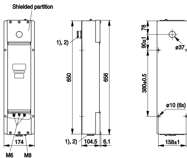
Drawing 4: B84299D2160B003 (2x16A), B84299D2320B001 (2x32A)
