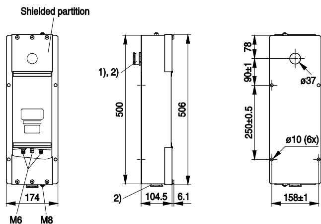
Drawing 2 - B84299D2060B003 (2x6A), B84299D2160B001 (2x16A)
