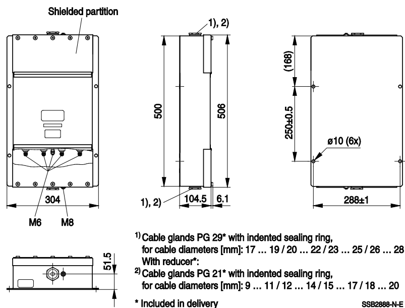
Drawing 7 - B84299C2060E003 (4x6A), B84299C2160E001 (4x16A)
