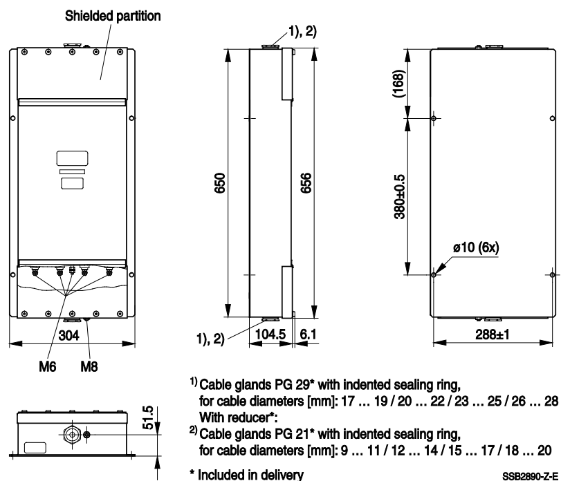
Drawing 11 - B84299C2320E001 (4x32A)
