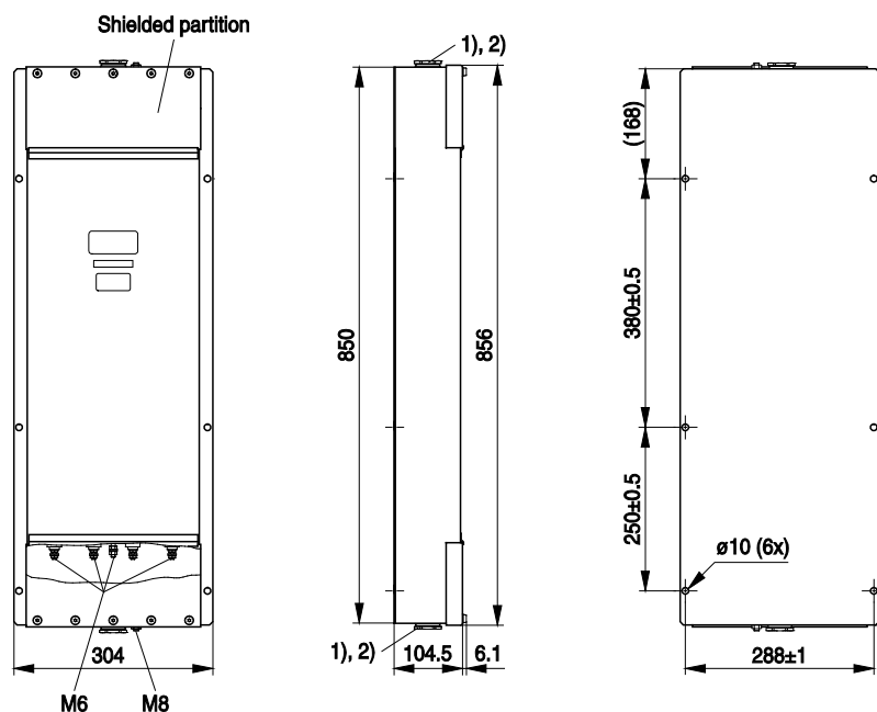
Drawing 13 - B84299C2320E003 (4x32A)
