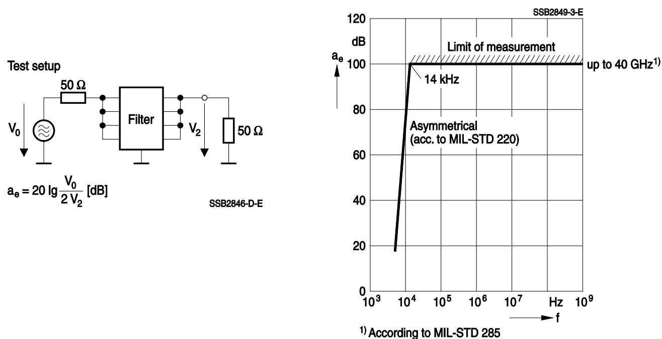
Attenuation diagram 2: Filters with 100dB from 14 kHz up to 40 GHz Insertion loss a_e as a function of frequency f (typical values at Z = 50 \text{ Ohm} )
