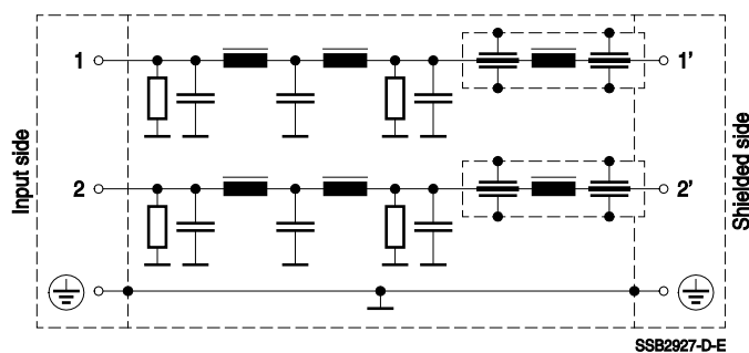
Circuit diagram 3: 2 line filters with 100dB from 14kHz
