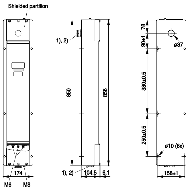
Drawing 6 - B84299D2320B003 (2x32A)
