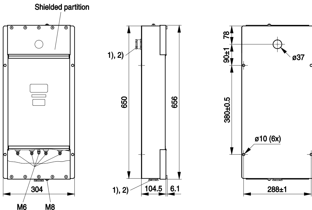
Drawing 10 - B84299D2160E003 (4x16A)
