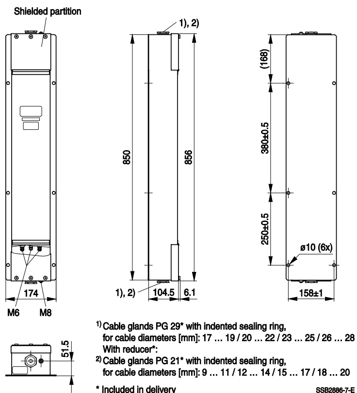
Drawing 5 - B84299C2320B003 (2x32A)
