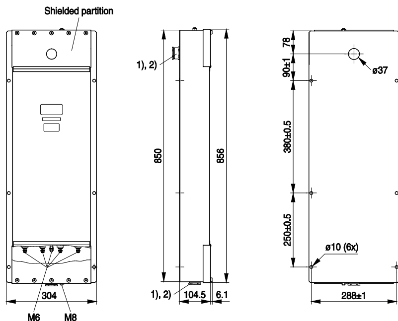
Drawing 14 - B84299D2320E003 (4x32A)
