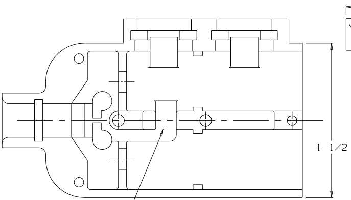
CHANNEL FOR SWITCH LEADS SHELL, HALF TJSS-106-2
