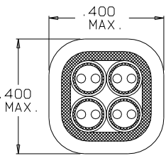
SECTION B-B STRAIN RELIEF CLAMP TJSS-106-6 AFTER CRIMPING SCALE 4:1
