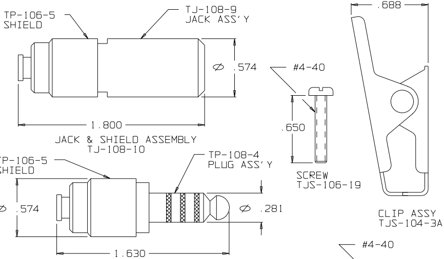
PLUG & SHIELD ASSEMBLY TP-108-6
