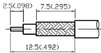
STRIPPING DIMENSION
