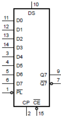
Figure 1. Logic symbol
