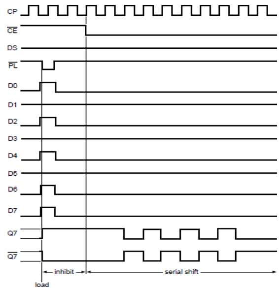
Figure 4. Timing diagram
