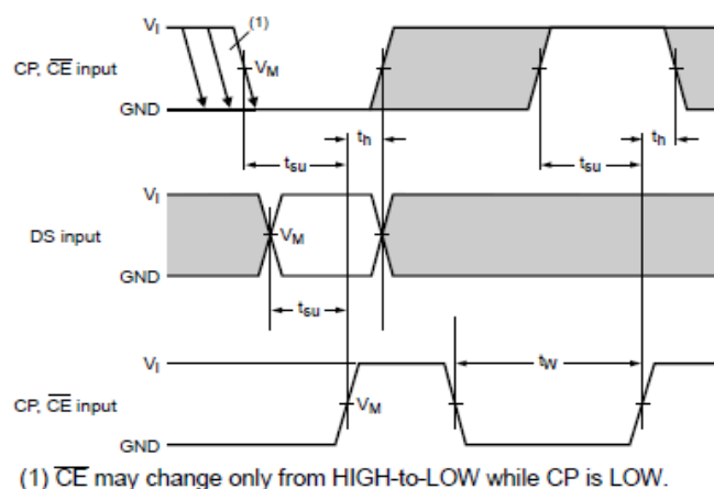
Figure 9. The set-up and hold times from the serial data input (DS) to the clock (CP) and clock enable ( \overline{\text{CE}} ) inputs, from the clock enable input ( \overline{\text{CE}} ) to the clock input (CP) and from the clock input (CP) to the clock enable input ( \overline{\text{CE}} )
