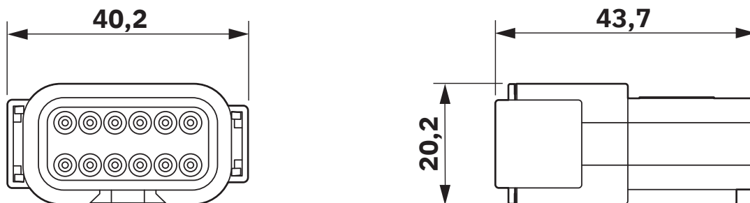
ATM04-12PA top view and side view
