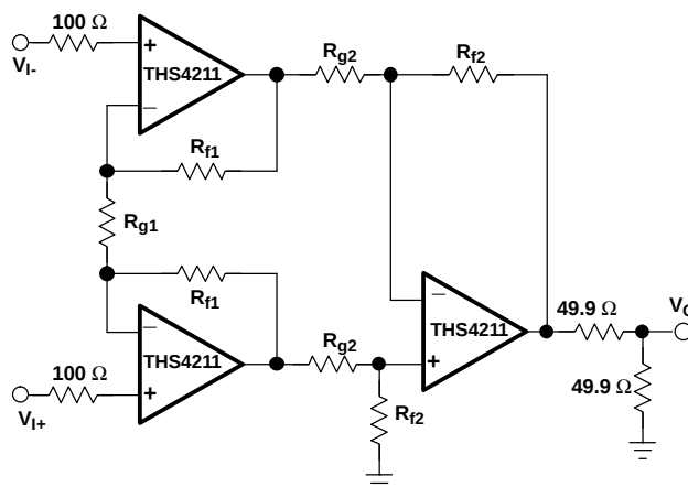
Figure 84. A High-Speed Instrumentation Amplifier
