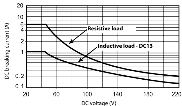
H 7S12* - Maximum DC breaking capacity - 7S.12
