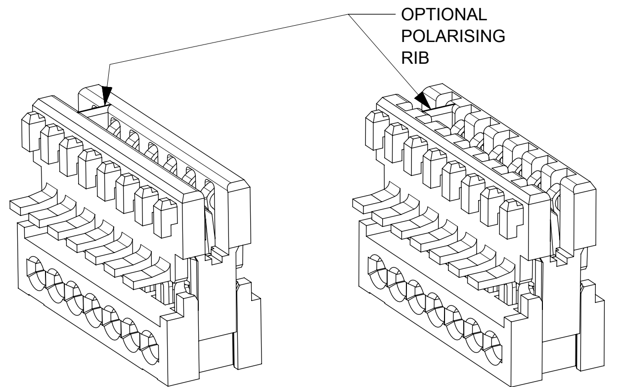
OPEN END WALLS WITH ZEUS OPTION.
