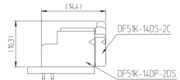
ENGAGEMENT FIGURE (2:1)
