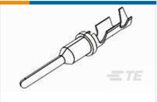
TE Part #1924463-3 PIN, SF, SIZE 16, 18-20 AWG, NI/SN
