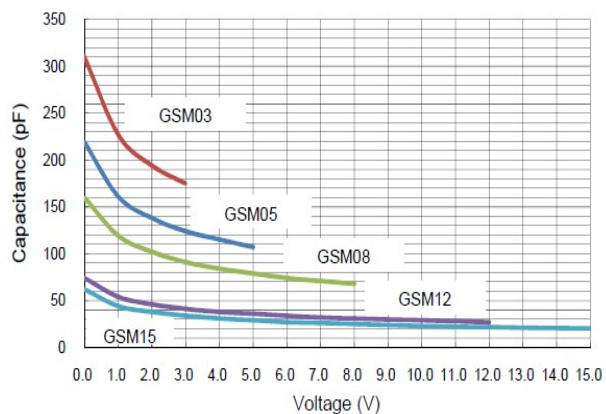
Fig 3 Voltage vs Capacitance
