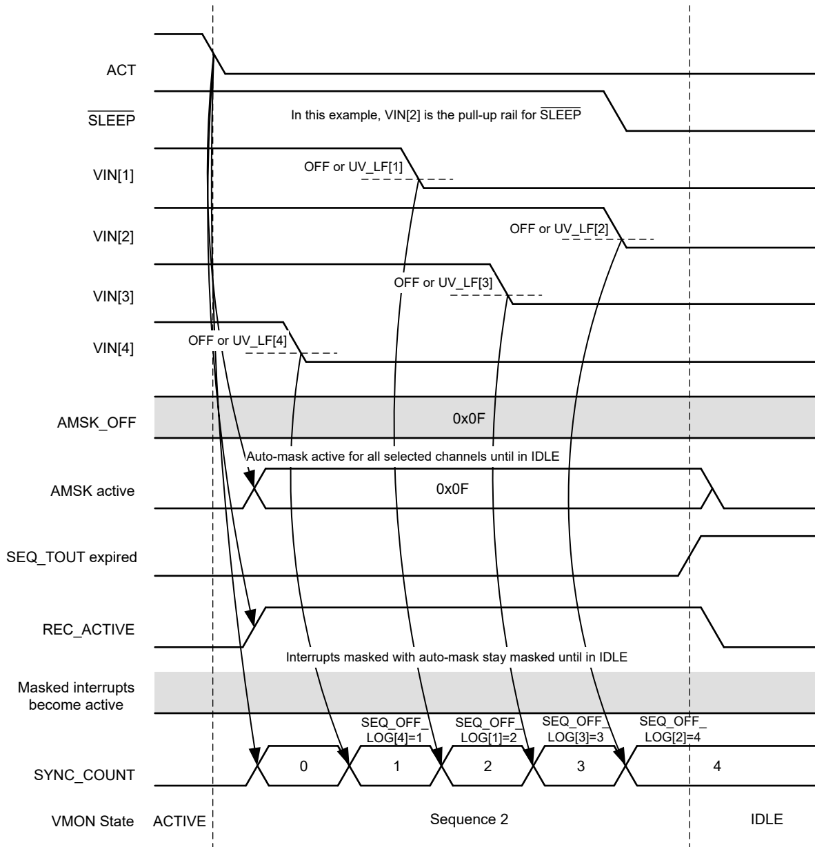
Figure 7-17. ACT 1→0 Transition
