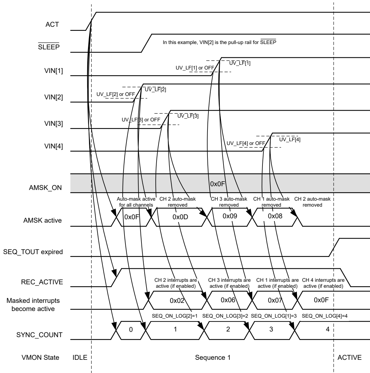
Figure 7-14. ACT 0→1 Transition
