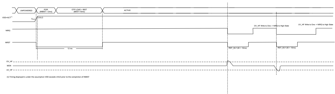
Figure 7-11. TPS389R06-Q1 Reset Timing diagram for voltage faults
