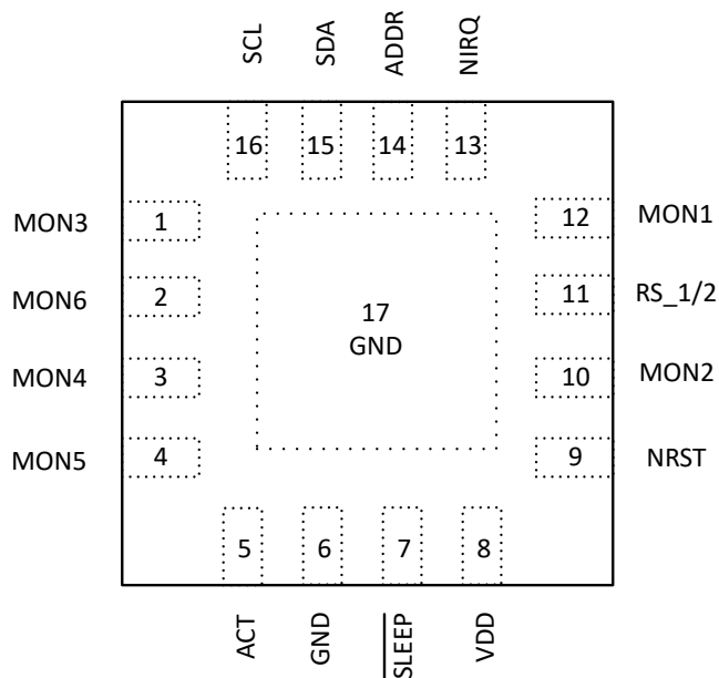
Figure 5-2. RTE Package 16-Pin WQFN TPS389R06-Q1 Top View
