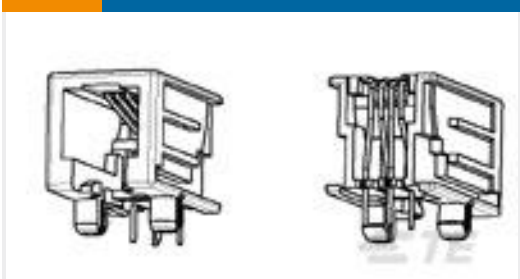
TE Part #1-1705950-1 Modular Jack SE, 6/6, Gold flash
