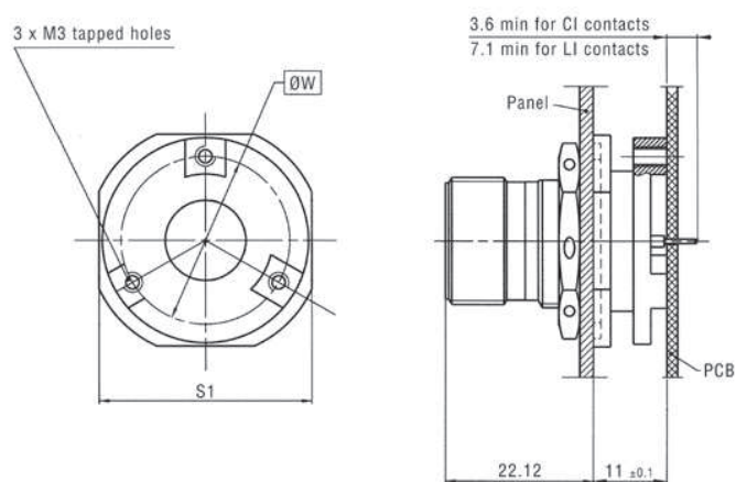
Jam nut receptacle (size 9 and 11)
