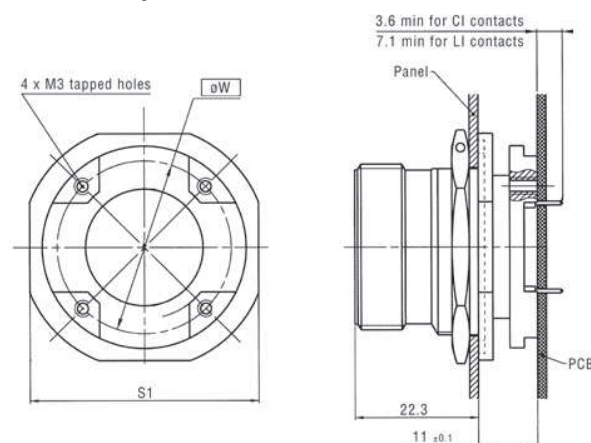
Jam nut receptacle (size 13 to 25)
