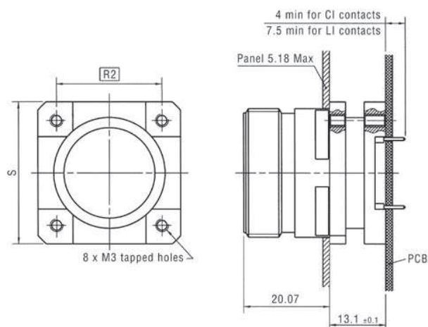
Square flange receptacle (size 9 to 25)
