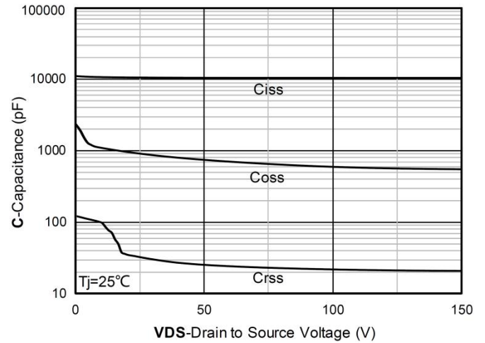
Capacitance Characteristics
