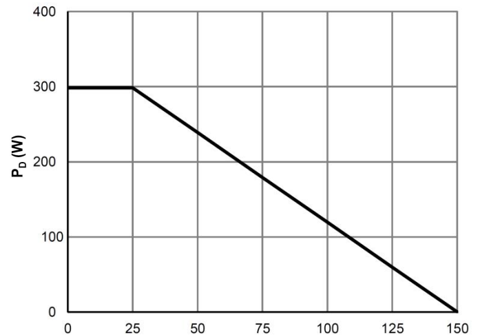
Power De-rating
