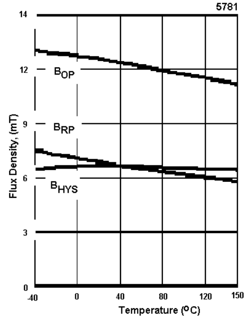
11.2. Magnetic Switch Points vs Temperature
