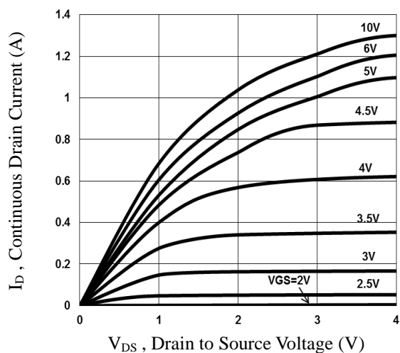
Fig.1 Output Characteristics
