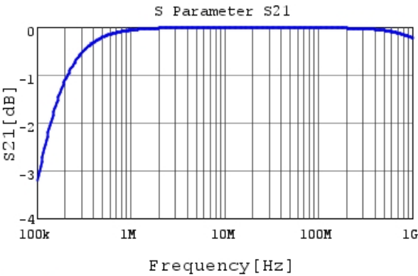
RHEL82A153K0A2H03B S21 DCOV, 25degC
