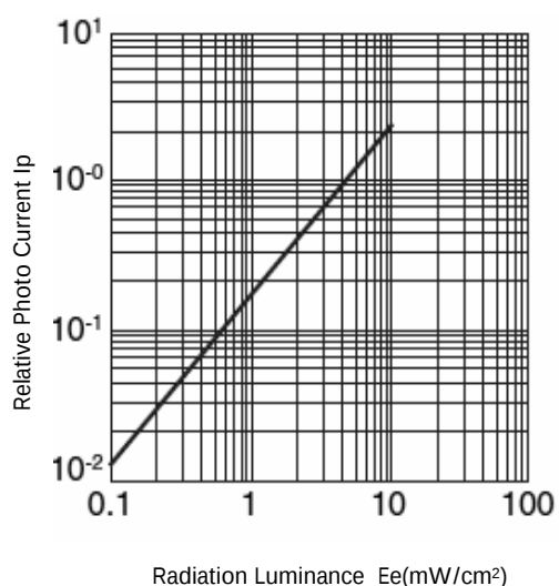
Radiation Luminance vs. Relative Photo Current Condition : T_a = 25 , V_R = 5V
