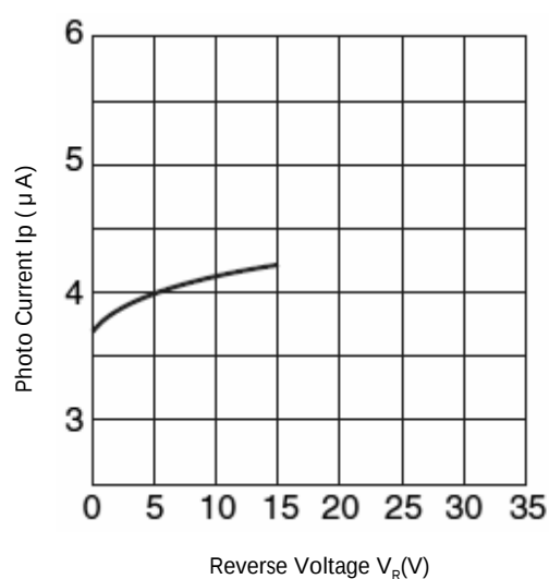
Reverse Voltage vs. Photo Current Condition : T_a = 25 , E_e = 5 \text{ mW/cm}^2
