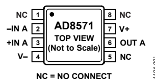
Figure 1. 8-Lead MSOP (RM Suffix)
