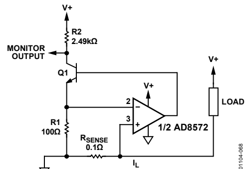
Figure 68. Low-Side Load Current Monitor
