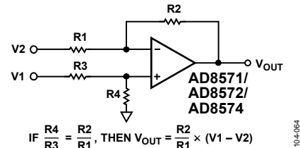
Figure 64. Using the AD857x as a Difference Amplifier
