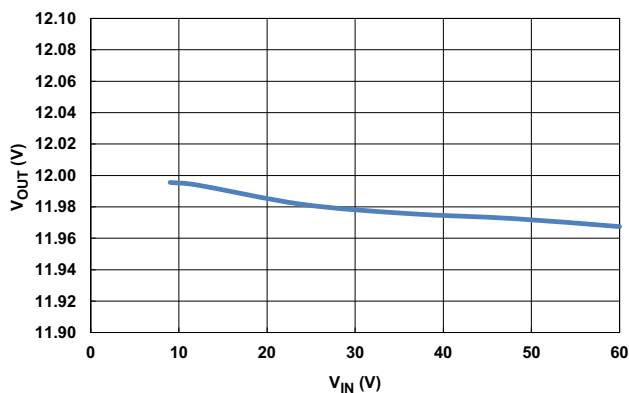
Figure 23. CCM Line Regulation at 10A Load +25°C
