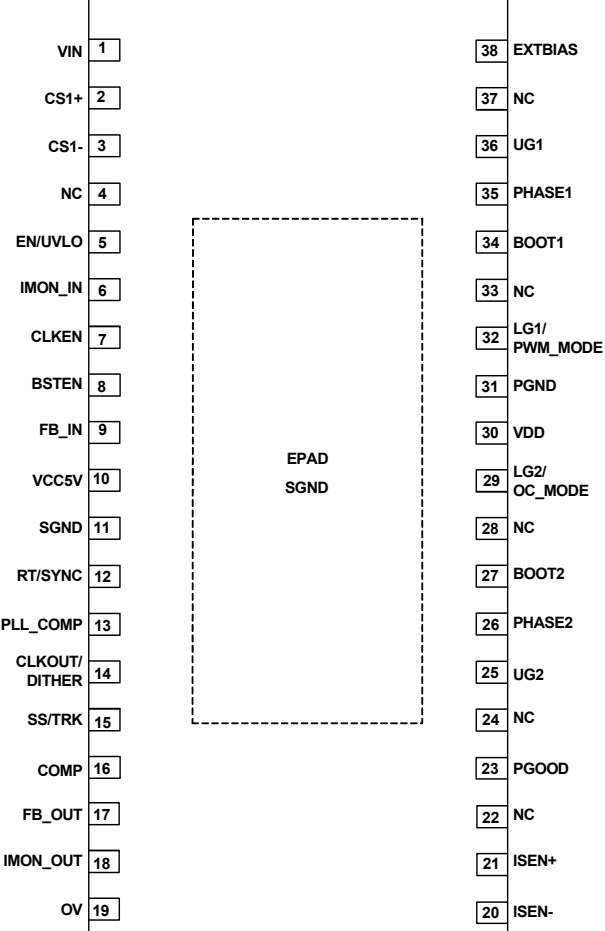
38 Ld HTSSOP Top View
