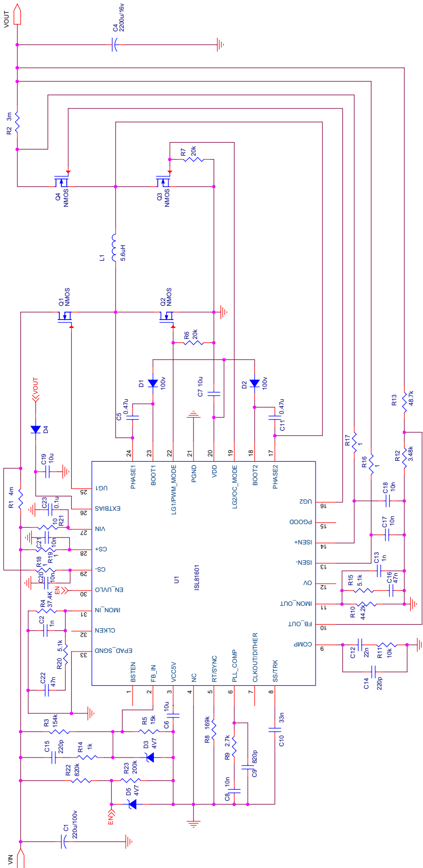
Figure 4. ISL81601EVAL1Z (VIN = 9V to 60V, VOUT = 12V, IOUT = 10A) Evaluation Board Schematic
