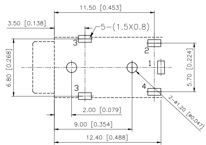
PCB Layout
