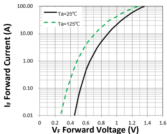
Figure 1. Forward Characteristic(typ.)
