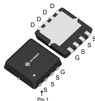
DFN3X3-8L (PowerPAK1212-8)
