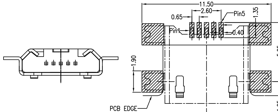
RECOMMENDED PCB LAYOUT PCB图仅供参考
